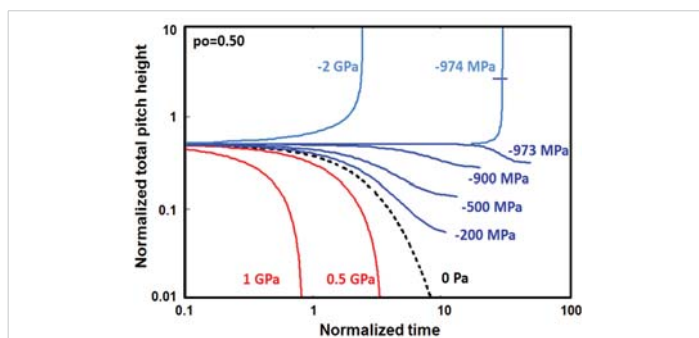
Figure 7: The unfolding of a Helical conformations, which have total pitch heights p_o / \ell_o \Rightarrow 0.50 below the critical value of p_{cr} = \ell_o / \sqrt{2} as an initial configurations under the action of the various positive and negative hydrostatic pressures. Threshold level is -973.4 MPa [ g_s = -292.014 \text{ erg/cm}^2 ] may be calculated from Eq. 5 by letting p = p_o . This initial configuration shows the nonequilibrium stationary states regime below the threshold level up the boundary of the aging region marked by dotted red line.
