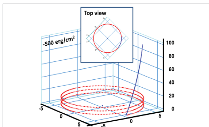
Figure 10: a) Perspective view: Helical conformation of \alpha -peptide at the stationary state is illustrated by (red dotted line), which has pitch height 5.4A^\circ , and radius 6A^\circ and 3 rings. When it is exposed to the spontaneous relaxation under the negative interfacial Gibbs free energy of g_s = -500 \text{ erg/cm}^2 [ p = -1.677 \text{ GPa} uniaxial tension, isobaric] the unfolding takes place (blue line), which is found to be 99.9% of the full transition b) Top View: Partial unfolding appears as an arc segment (blue color) having \Theta = 49.5^\circ azimuthal angle with a torsional inclination angle of \beta = 2.563^\circ . That should be zero if one takes final total pitch height as p = \ell_o .
