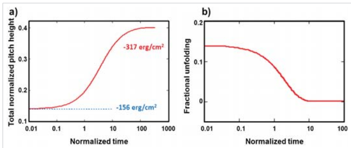
Figure 2: a) The unfolding of a Helical conformation 3.6_{13} with expansion in the stability region of the negative hydrostatic pressure and interfacial free energy manifold driven by the stored elastic torsional energy in collaboration with the critical interfacial Gibbs free energy. b) Isochoric unfolding at absence of the surface and hydrostatic pressure terms. It is solely driven by the stored torsional elastic energy, which is about 3 eV/molecule.
