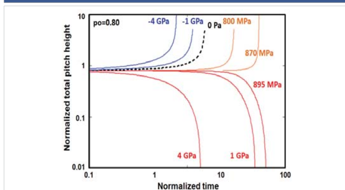
Figure 8: The unfolding of a Helical conformation, which has an initial pitch height p_o / \ell_o \Rightarrow 0.80 , above the critical value of \hat{p}_o > 1/\sqrt{2} , shows two distinct regions under the hydrostatic pressure separated by a threshold level. Above which it is completely in the state of instability, which is ending up with the complete unfolding with zero elastic rotation and bending energies. The other region shows stability with decreasing in pitch height up to the flat configuration. The hydrostatic pressure in this regime decreases the relaxation life time in the stability domain. This just the opposite in the case of dynamic instability regime, where it increases. Threshold level is 872.1 MPa [ g_s = 261.014 \text{ erg/cm}^2 ] may be calculated from Eq. 5.
