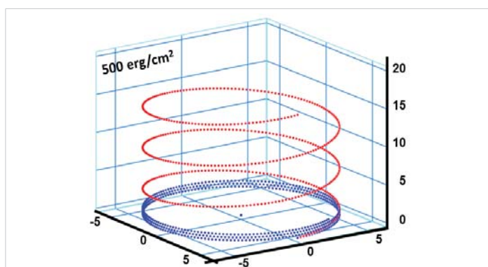
Figure 9: Helical conformation of \alpha - peptide at the stationary state is illustrated by (red dotted line), which has pitch height 5.4\text{\AA} , and radius 6\text{\AA} and 3 rings. When it is exposed to the spontaneous relaxation under the positive interfacial Gibbs free energy of g_s = +500 \text{ erg/cm}^2 [= 1.677GPa] under 1 ATM pressure (isobaric) then the unfolding takes place (blue line), which is found to be 86.4% of the full transition, having \Theta = 3.077 cycle.
