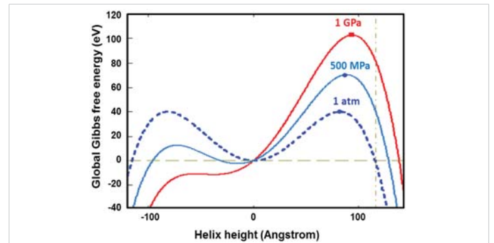
Figure 3: Global Gibbs free energy of \alpha -Helix 3.6_{13} is plotted with respect to the total pitch height for various values of the applied stress in absence of the interfacial Gibbs free energy. Eq. (10) operates only in domain, where \ell_o \geq p \geq 0 , the rest is given for the illustration. One would have very similar plots for the positive interfacial free energies. The negative gradients of these curves give the directions of the natural time evolutions of helical conformation.
